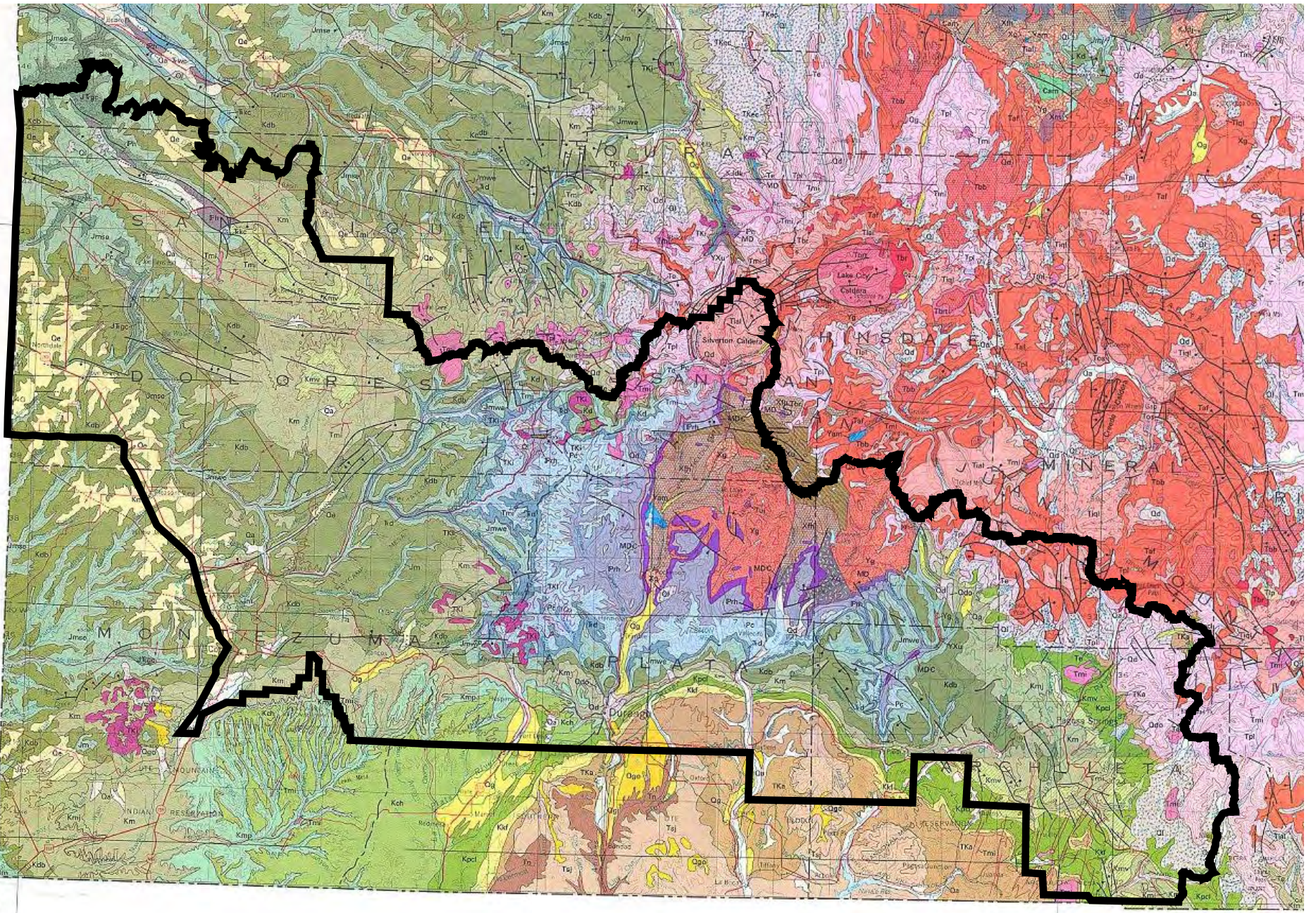
FIGURE 5 GEOLOGY OF THE RFD AREA AND ADJACENT LANDS
